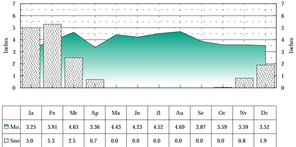
Asheville Area - Average Monthly Precipitation
