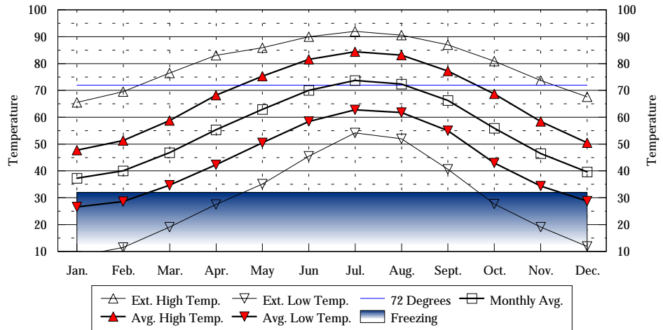
Asheville Area - Average Monthly Temperature, (F)
