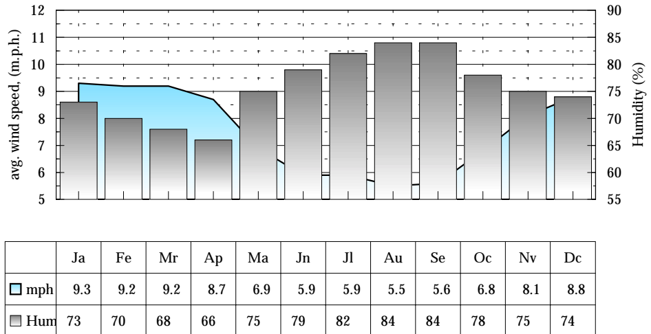
Asheville Area - Average Monthly Wind Speed & Humidity
