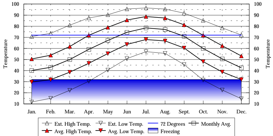
Raleigh-Durham Area - Average Monthly Temperature, (F)
