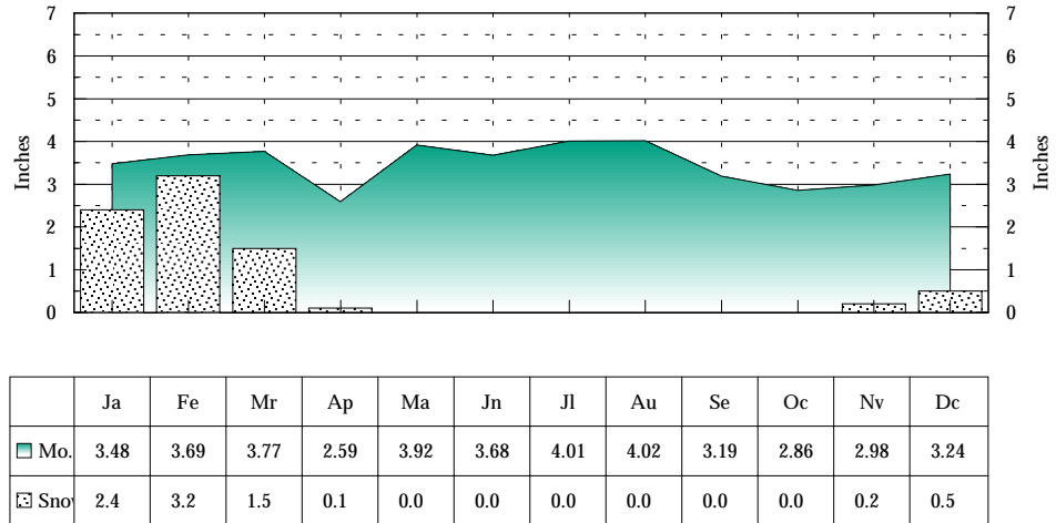
Raleigh-Durham Area - Average Monthly Precipitation
