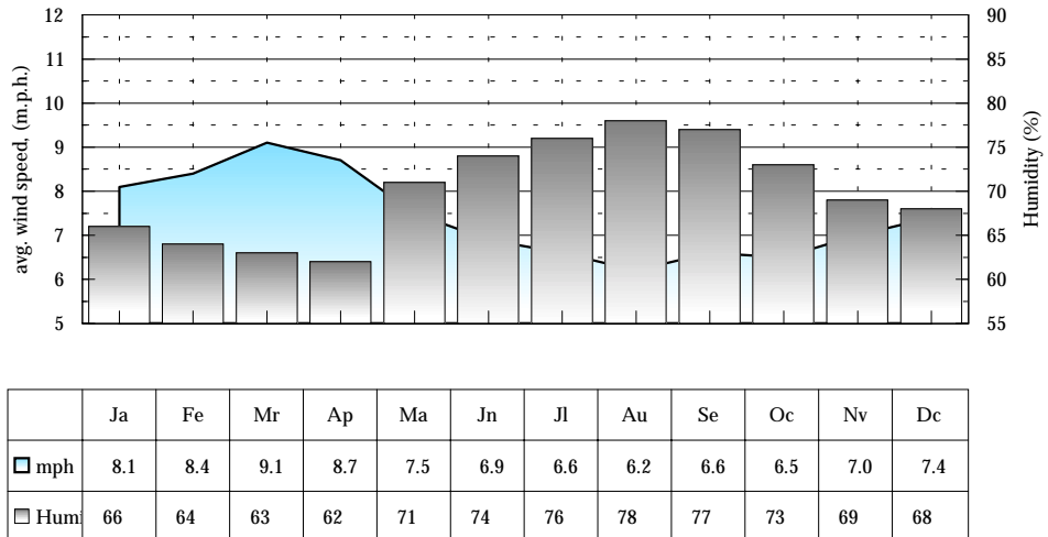
Raleigh-Durham Area - Average Monthly Wind Speed & Humidity
